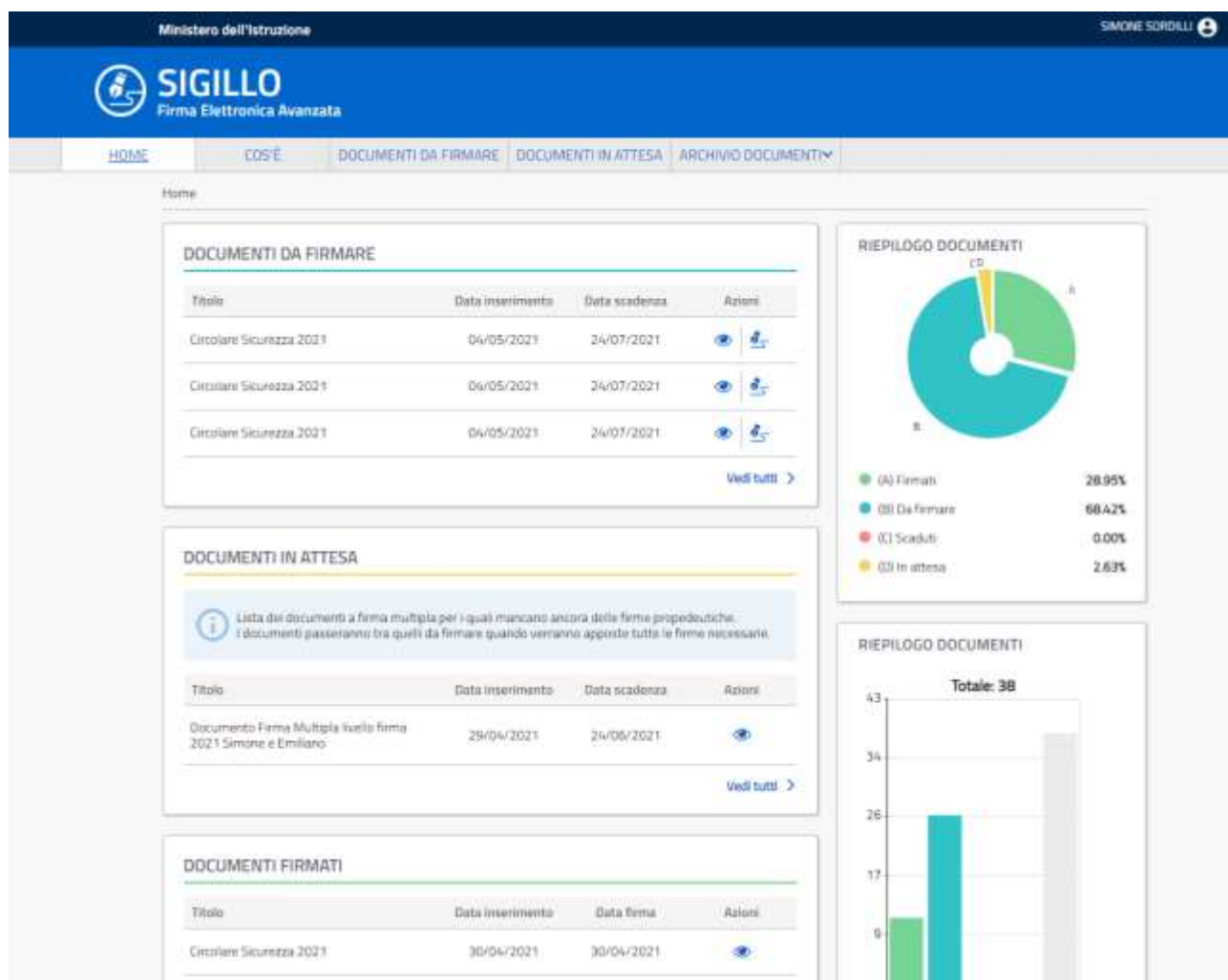
Figura 2 – Home Page
